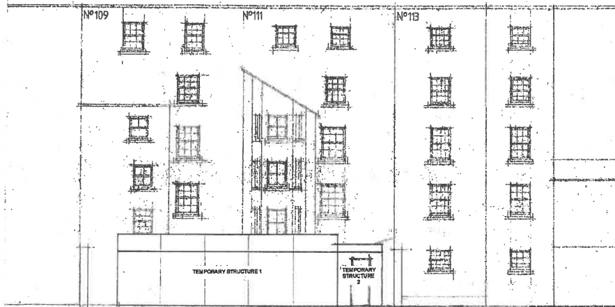
NORTH WEST ELEVATION TO MONTPELLIER STREET 1:100 at A3
